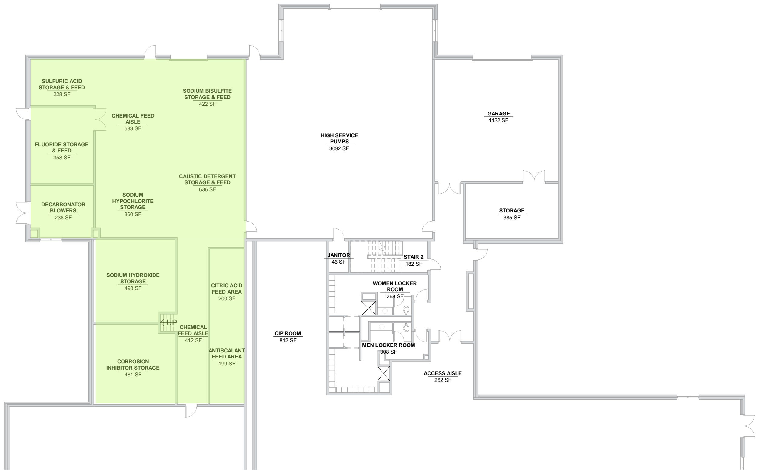
① OPERATING FLOOR 1A - PROGRAM 1/16" = 1'-0"
