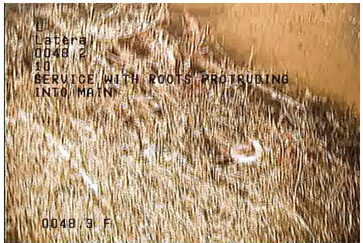
L - Lateral @ 48.2 ft. SERVICE WITH ROOTS PROTRUDING INTO MAIN
