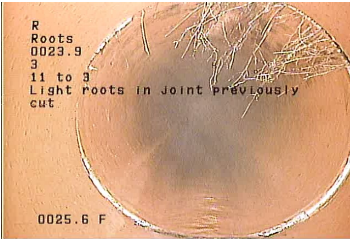
R - Roots @ 23.9 ft. Light roots in joint previously cut
