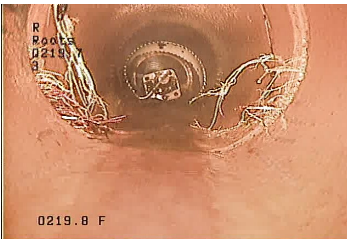
R - Roots @ 219.7 ft.
