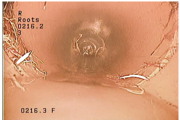
R - Roots @ 216.2 ft.
