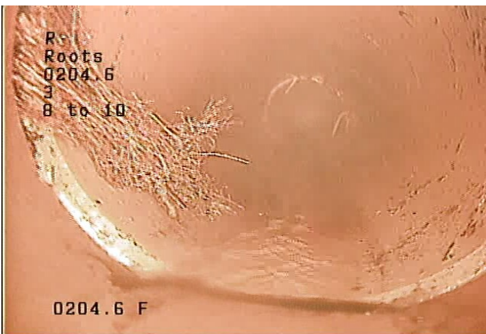
R - Roots @ 204.6 ft.
