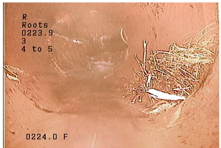
R - Roots @ 223.9 ft.
