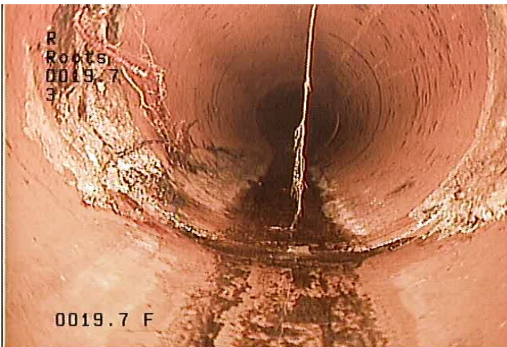
R - Roots @ 19.7 ft.
