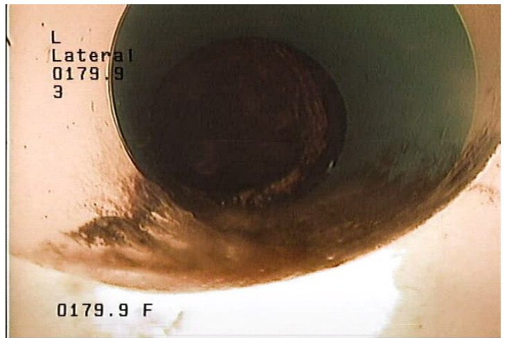
L - Lateral @ 179.9 ft.
