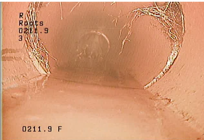
R - Roots @ 211.9 ft.
