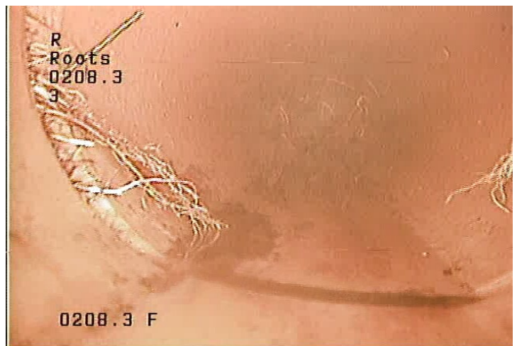
R - Roots @ 208.3 ft.
