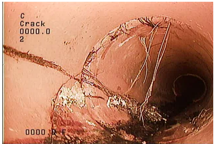
C - Crack @ 0.0 ft.
