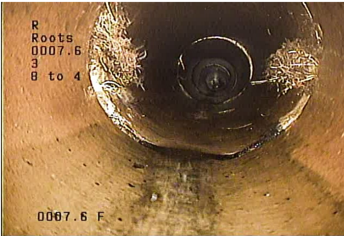
R - Roots @ 10.5 ft.
