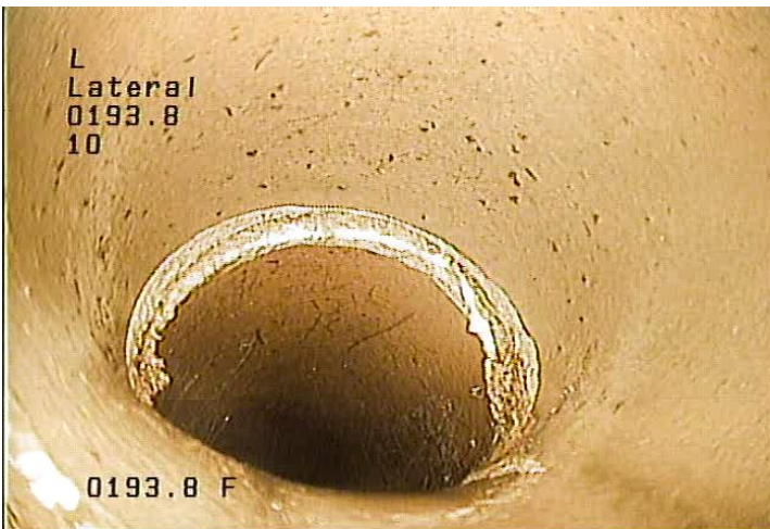
L - Lateral @ 193.8 ft.
