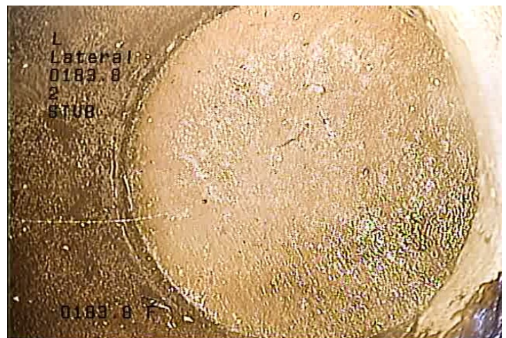
L - Lateral @ 183.8 ft. STUB
