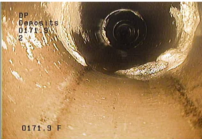
DP - Deposits @ 171.9 ft.
