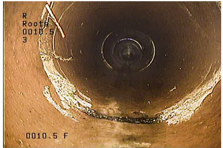
C - Crack @ 11.3 ft.
