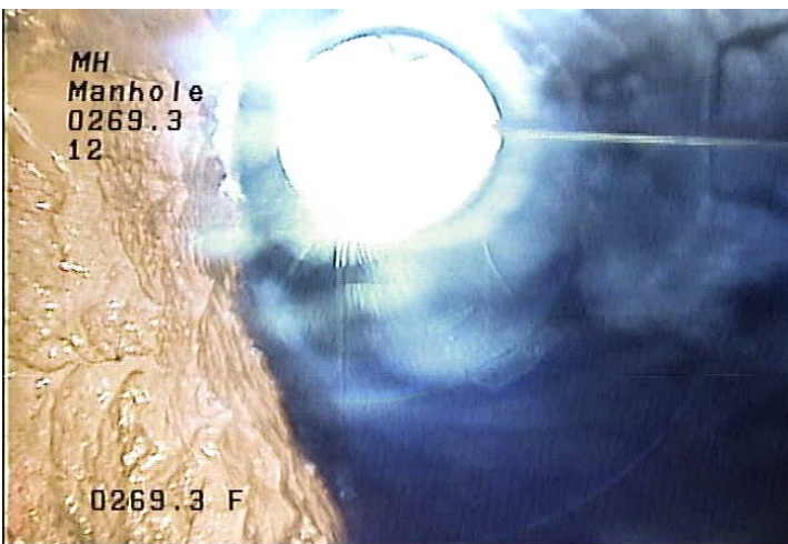
MH - Manhole @ 269.3 ft.
