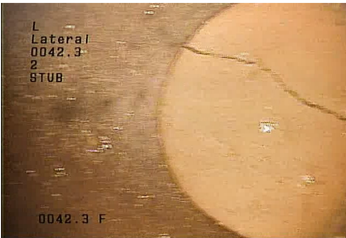
L - Lateral @ 42.3 ft. STUB
