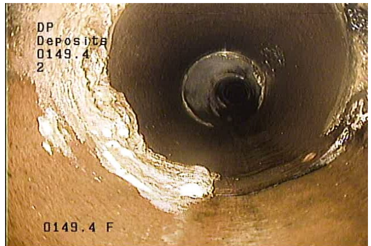
DP - Deposits @ 149.4 ft.
