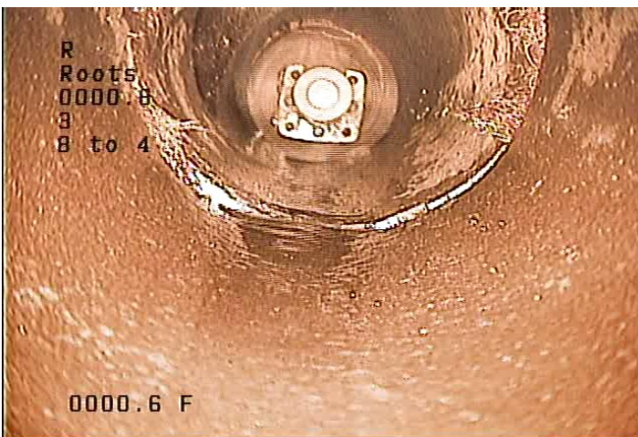
L - Lateral @ 3.5 ft. STUB
