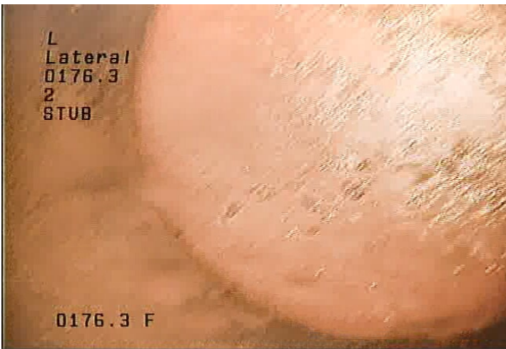
L - Lateral @ 176.3 ft. STUB
