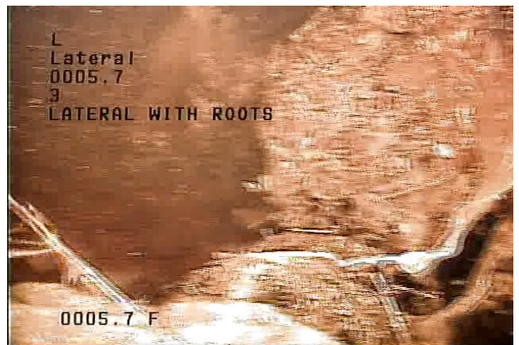
L - Lateral @ 5.7 ft. LATERAL WITH ROOTS
